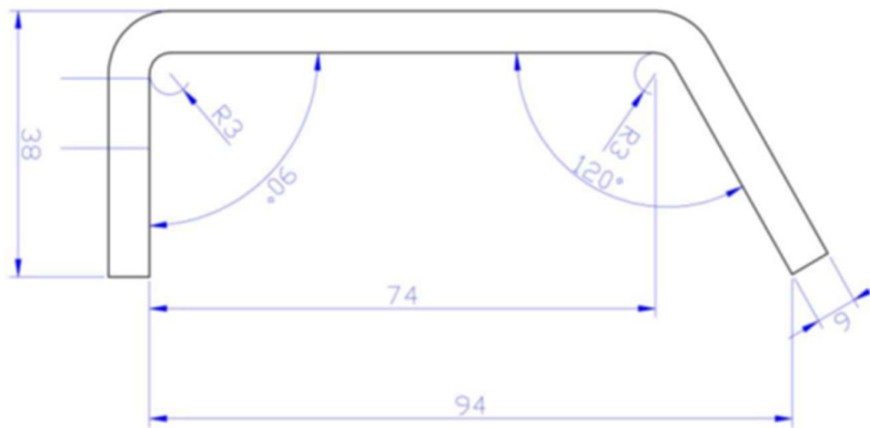
Profile of Blank Clamp Bar
